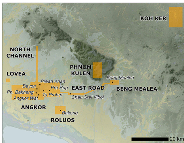
Fig. 1. An overview of the lidar acquisition areas in northwest Cambodia (background data courtesy of the Shuttle Radar Topography Mission).
